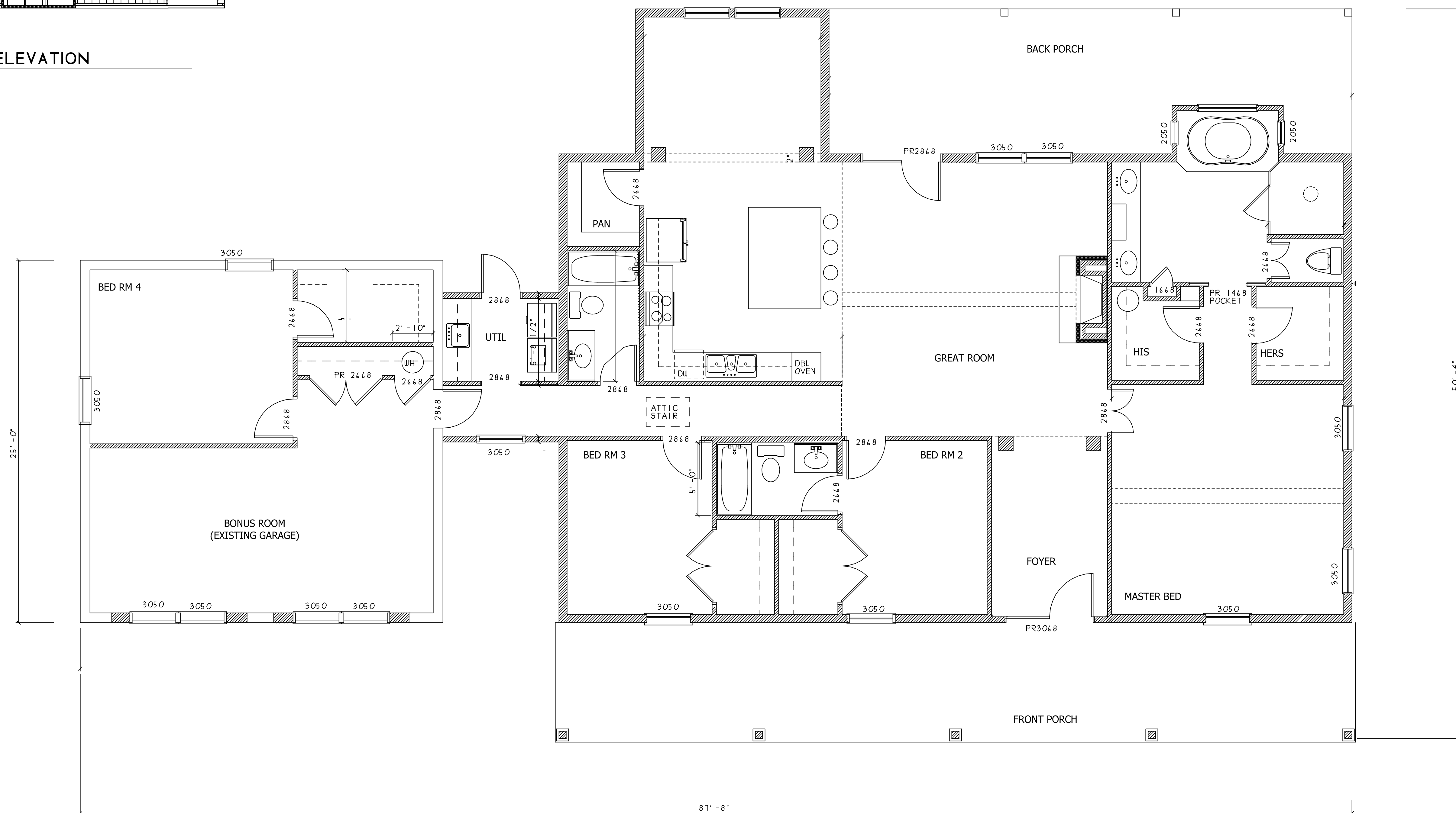
FLOOR PLAN
