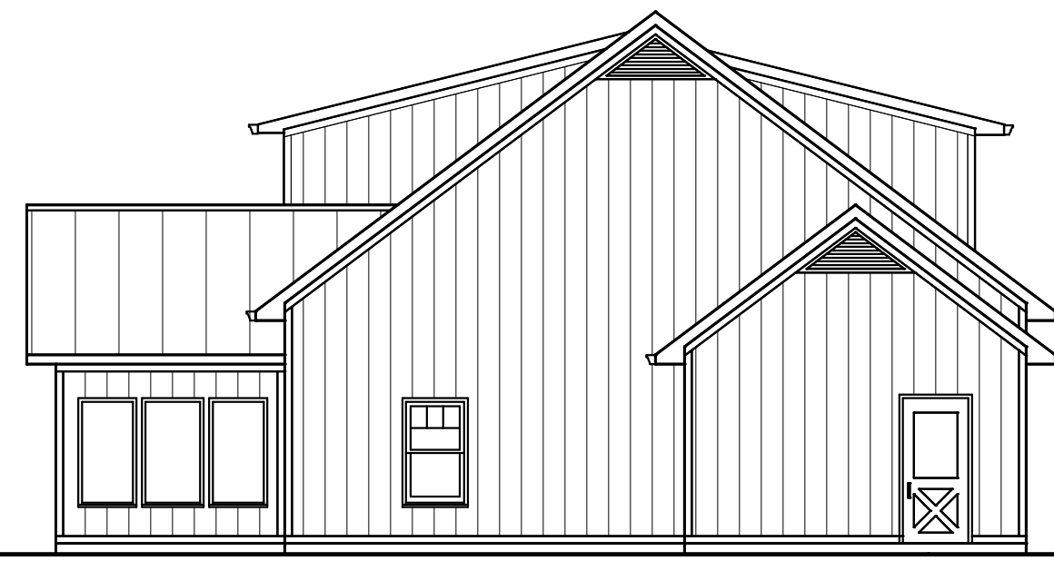
LEFT ELEVATION
